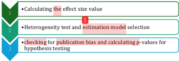
Figure 1. Data analysis procedure in meta-analysis
