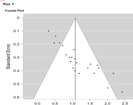
Figure 2. Funnel Plot Standadr Error
