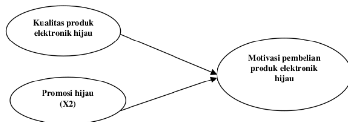
Gambar 1. Rerangka Model
