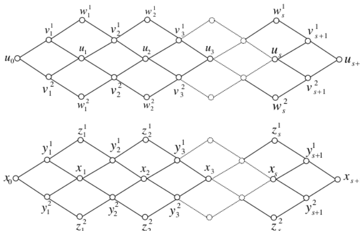
Figure 3. Combined string graphs R(s) \cup R(s)
