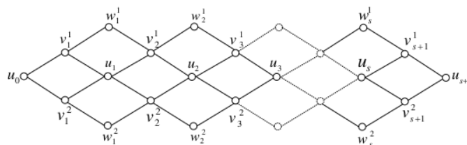
Figure 1. string graph R(s)
