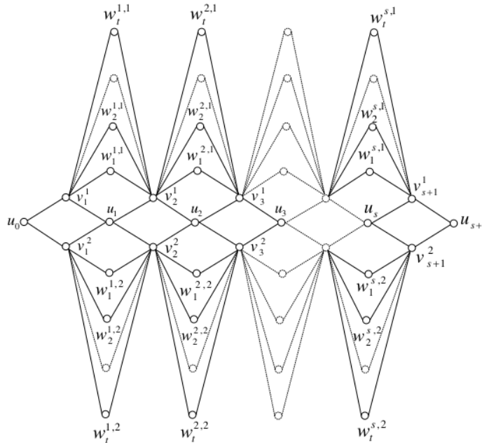
Figure 5. Graph of a multiple string R(s, t)
