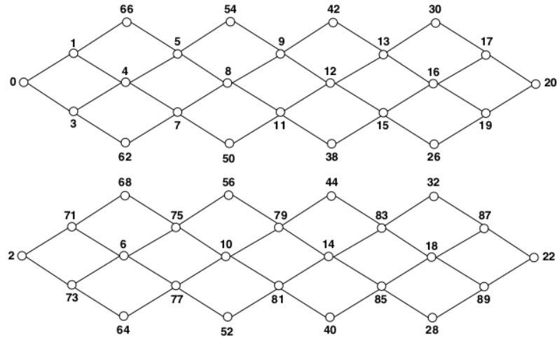
Figure 4. Combined string graphs R(4) \cup R(4)
