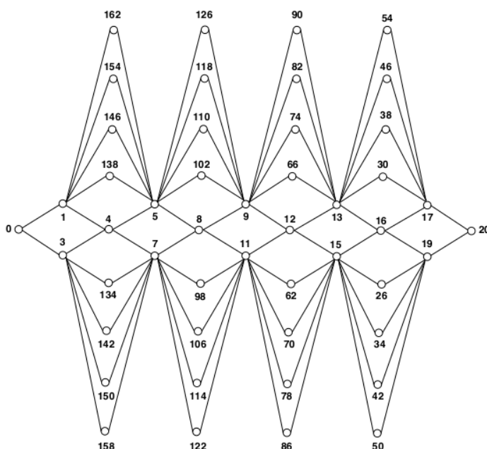
Figure 6. The graph of a multiple string R(4, 3)
