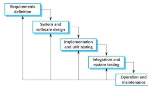
Gambar 1. Metode Waterfall
