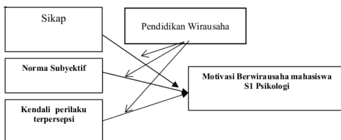
Gambar 1. Rerangka model
