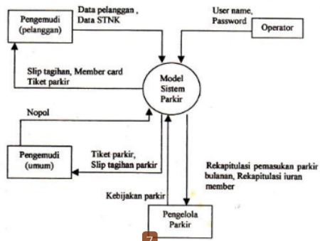
Gambar 1. DFD Level 0
