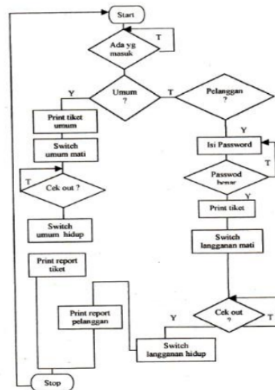
Gambar 4. Flow Chart
